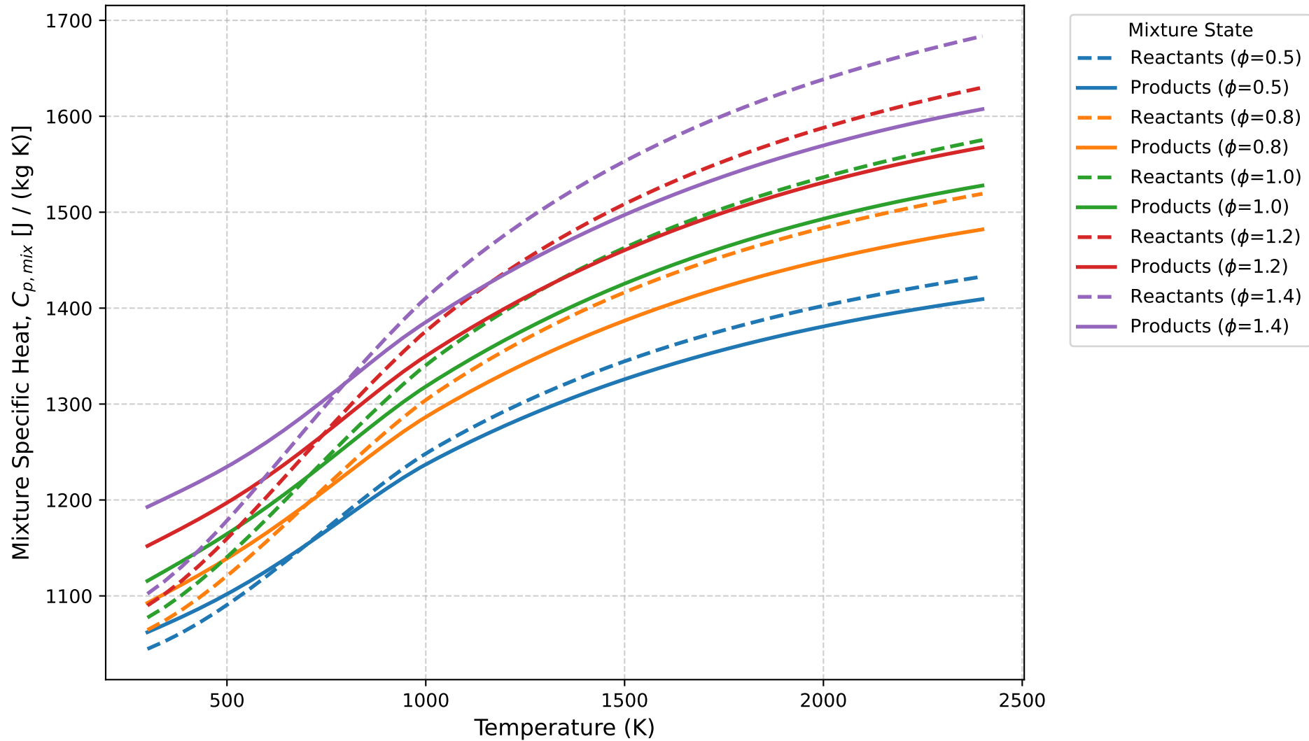
Variation of Mixture C_p for Methane ( CH_4 )-Air (Frozen Products)
